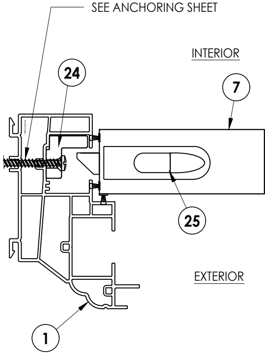
DETAIL 1
