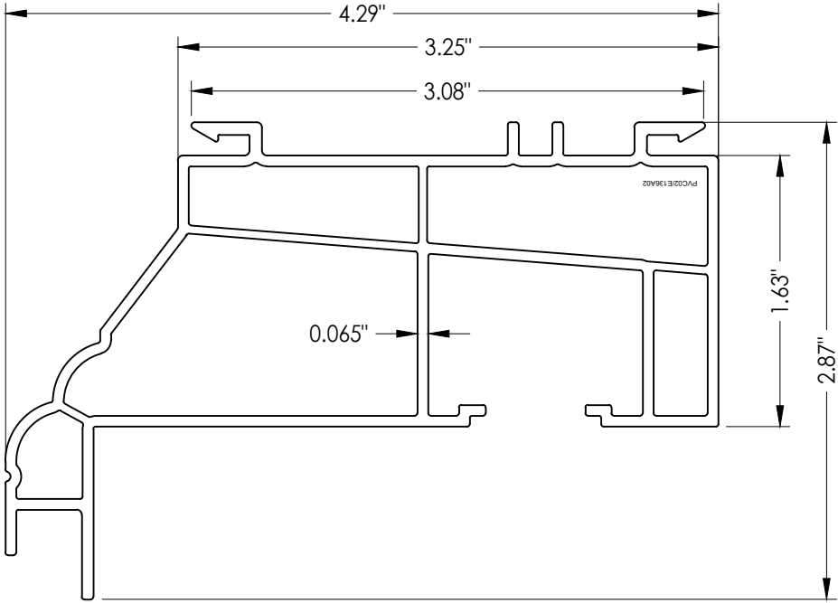
2 HEAD
