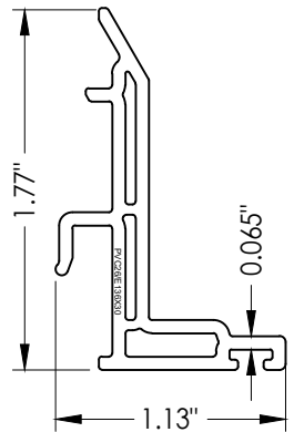
14 HEAD POCKET INSERT
