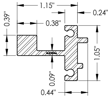
12 REINFORCEMENT
