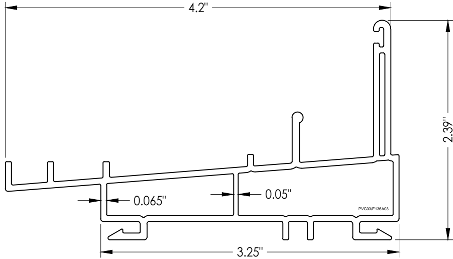
3 SLOPED SILL "DH30I"
