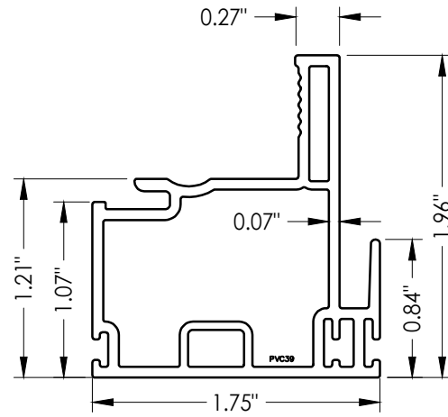
6 KEEPER RAIL
