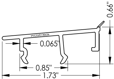
15 SLOPED INSERT
