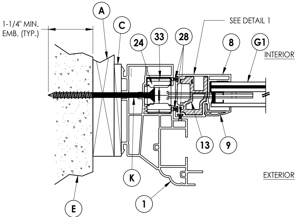
3 HORIZONTAL CROSS SECTION 2 Shown w/ 1X Buck
