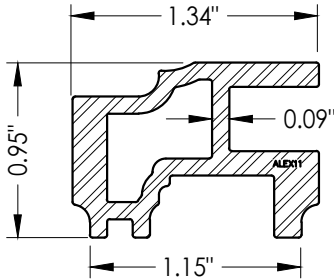
13 REINFORCEMENT
