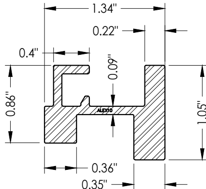
11 REINFORCEMENT
