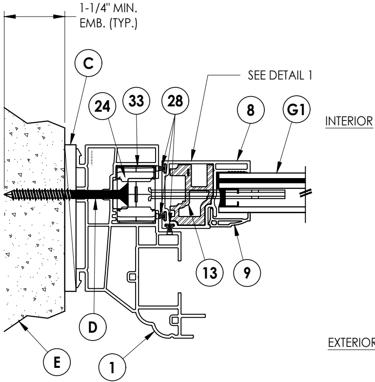
2 HORIZONTAL CROSS SECTION 2 Shown Direct to Masonry
