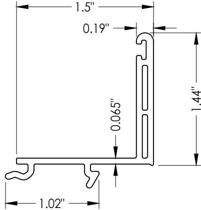
4 SILL ADAPTER
