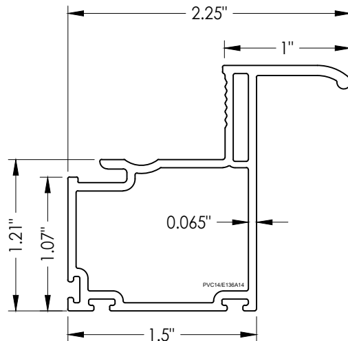
5 LIFT RAIL
