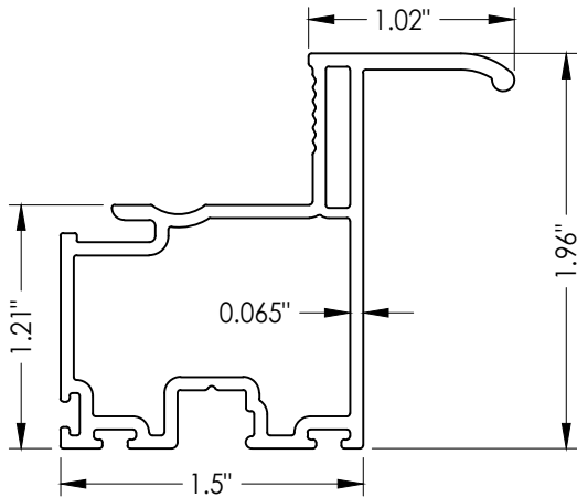
10 LIFT RAIL
