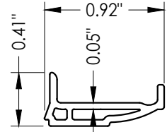
9 GLAZING BEAD
